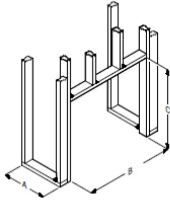
Rough-In Framing Dimensions
