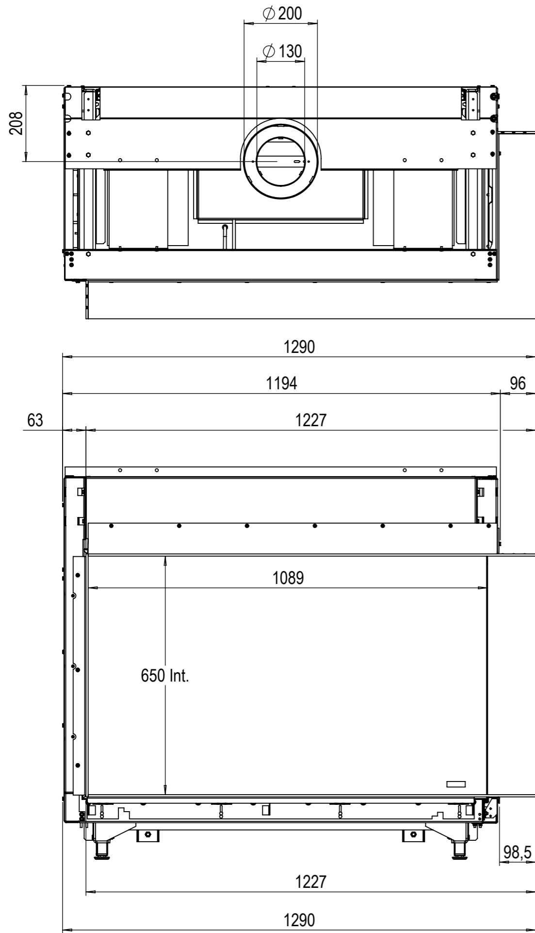
Dimensional drawing 1050-650 - II R (100)
